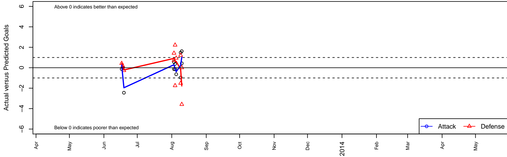
PAC San Jose Atlas B98 Dots are actual minus expected GF (blue circles) and GA (red triangles). Blue line is smoothed change in attack strength. Red is smoothed change in defense strength.
